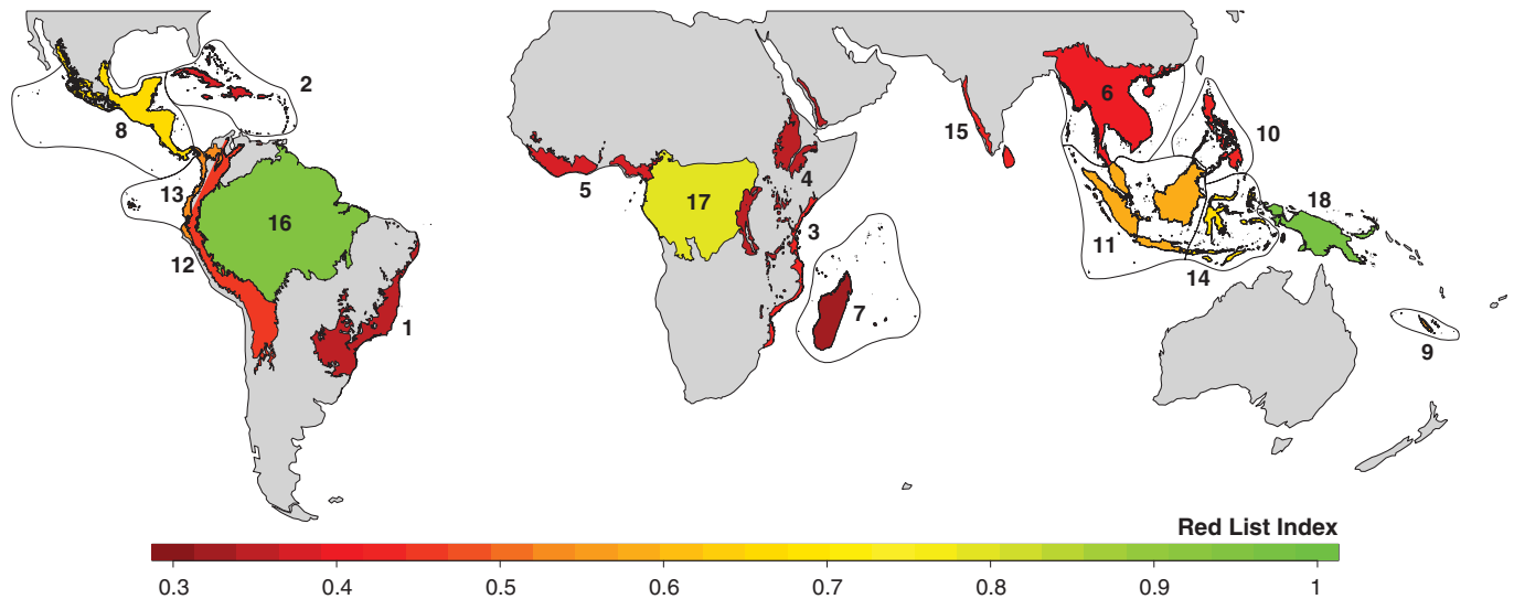
Fig. 4. Predicted RLI values for the 18 main tropical forest areas of the world. Predictions are based on the relationship between population size reductions and habitat loss, which could be obtained for all forests from forest cover maps and reports of their number of endemic species. Thus, these predictions are based solely on the population size reductions (i.e., IUCN
