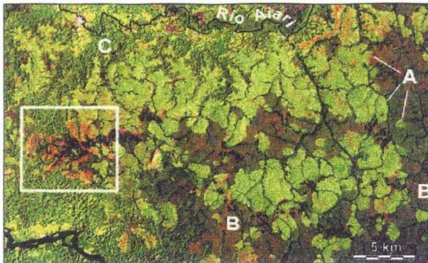
Figure 1. Burn scars on terra firme of upper Rio Negro: A) Low regrowth forest on sandy soil burn scars, some delimited by natural fire breaks; B) Tall unburned campinarana forest on sandy soil; C) Tall unburned dense forest on clay soil, light green areas along Aiari River are swidden fallows on same soil; White box: vegetation type “A” deleafed by recent ground fire. Landsat TM color composite of bands 3,4, & 5 (B,G,R), 29 Dec 1993, from INPE.
