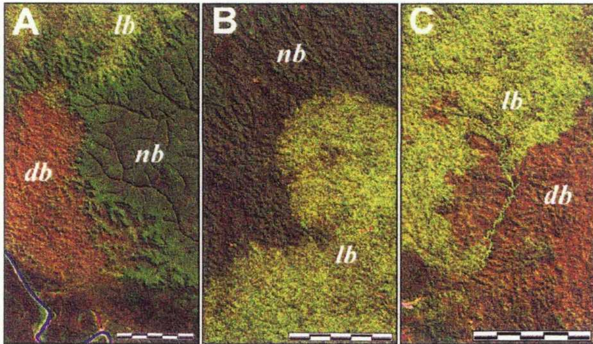
Figure 6: A): limit between bamboo and non-bamboo forests determined by soil/topography, B) rounded limit unrelated to topography; C) rounded limit between living and synchronously dying bamboo populations, partially coincident with natural fire break (stream). Scale bars are 5 km. db : forest with dead bamboo, lb : forest with living bamboo, nb : non-bamboo forest. Landsat TM color composites of bands 3, 4, & 5 (B,G,R), scene 002/066 of 04 August 1988, from INPE.
