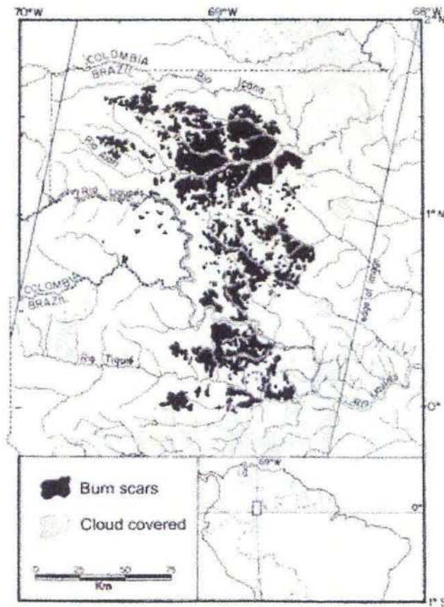
Figure 2. Burn scars covering 5,000 km 2 in two Landsat TM images of upper Rio Negro.
